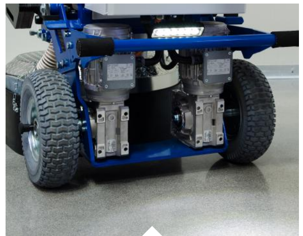
Powerful drive motors (SX and Self Track Version).
