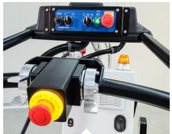
Controls for handling (Self Track Version).
