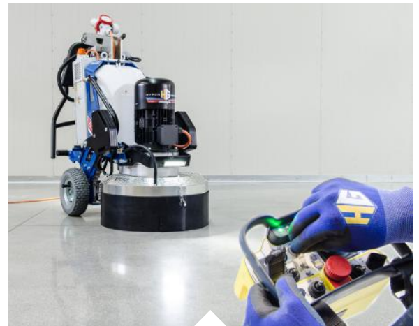
Remote controlled (SX version).
