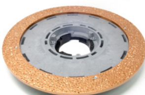
Tytan Ring \varnothing 430mm To remove old cement glues, resins, scratch floors and remove creases and excess thicknesses
